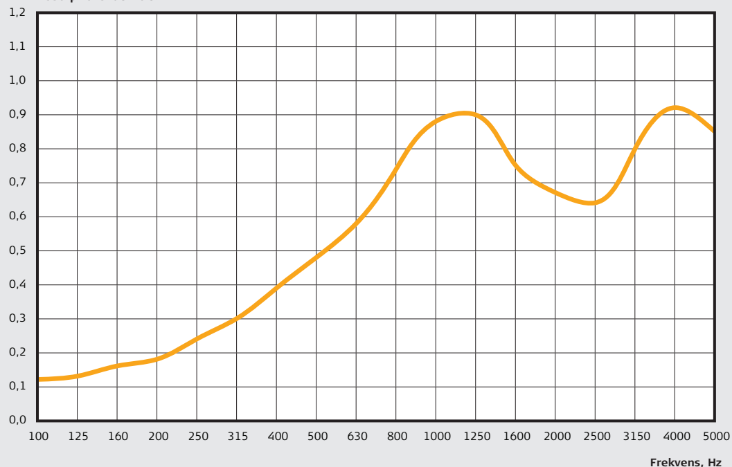
Absorptionskoefficient \alpha
